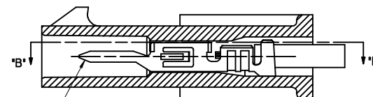
SECTION "D"- "D" WITH TERMINAL NO SCALE
