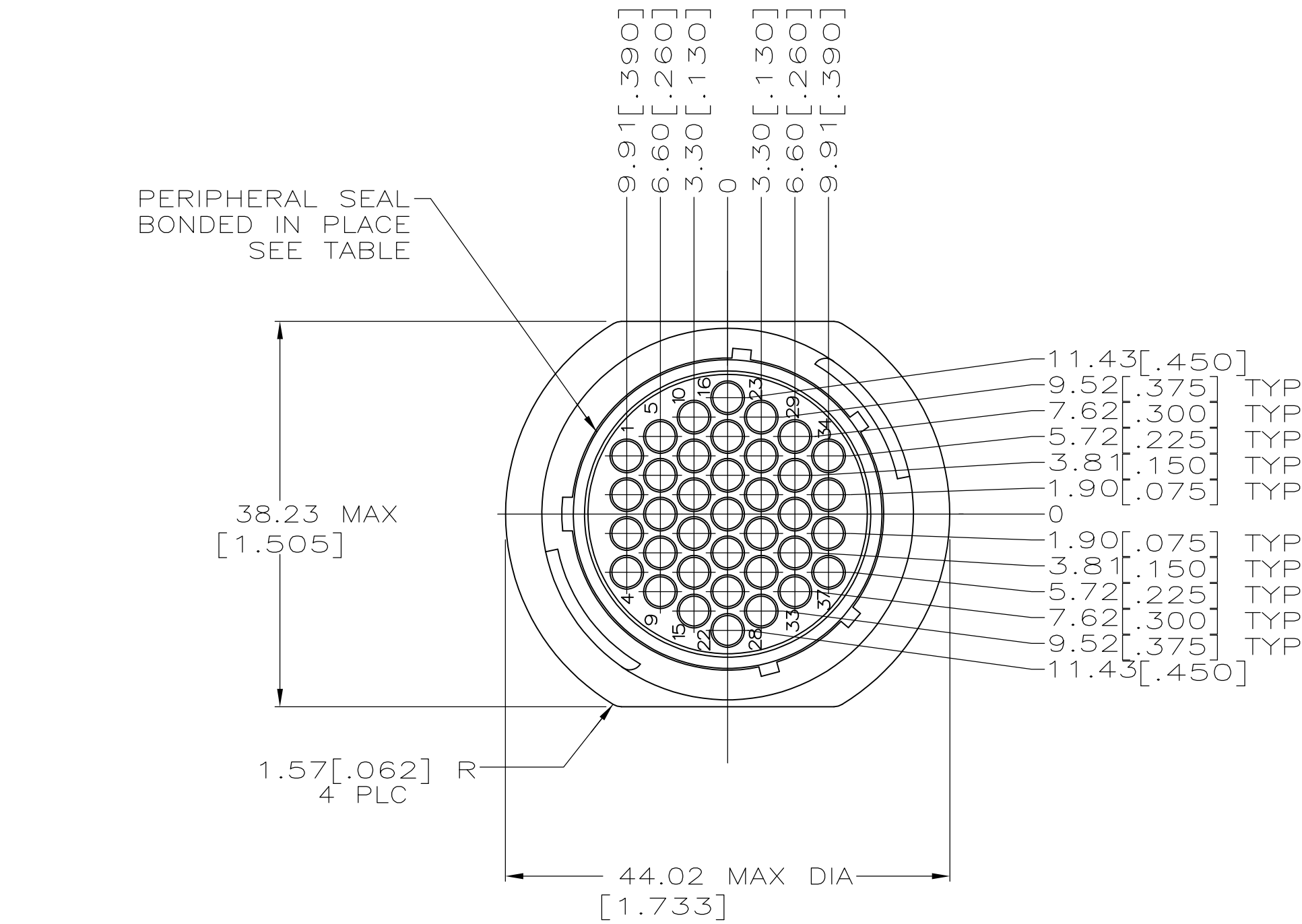
DETAIL B
