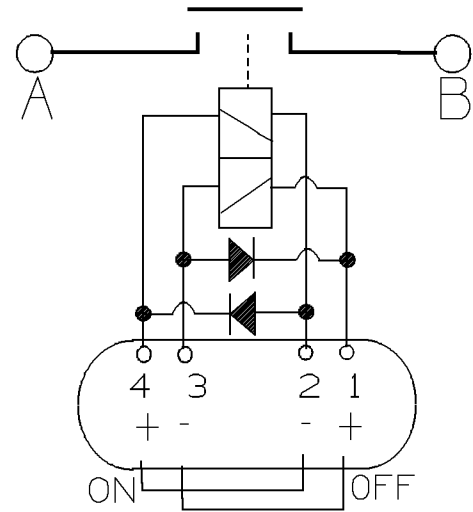
Pin Assignment
