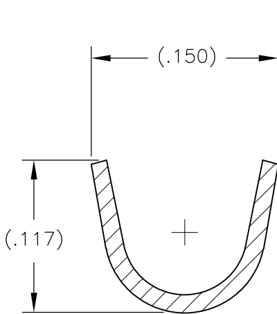
SECTION X-X
