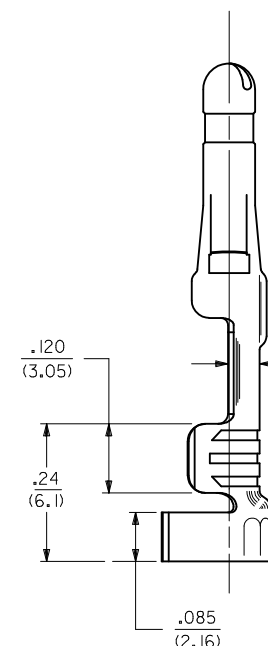
SECT. "B-B"
