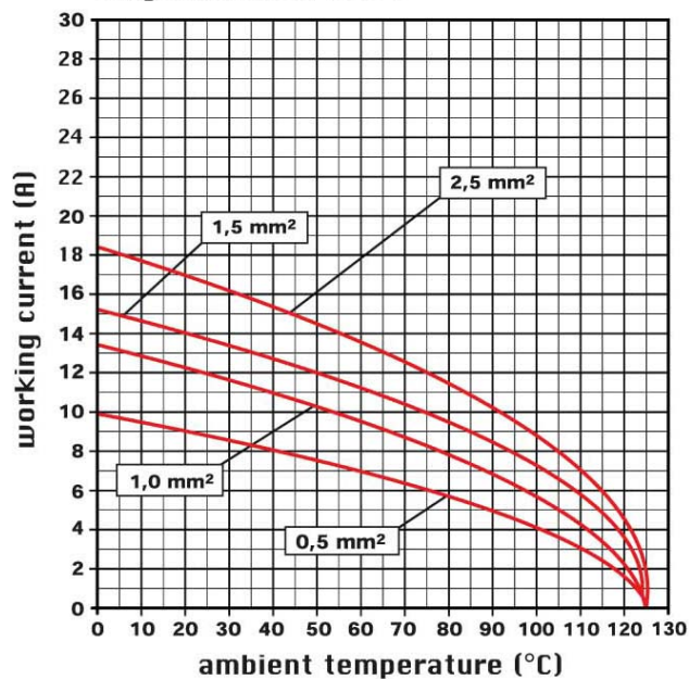
diagram CSH 24 poles
