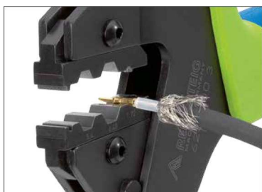
Innenleiter-Crimp Inner conductor crimp
