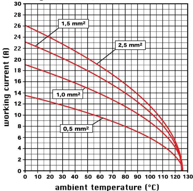
diagram CSH 06 poles
