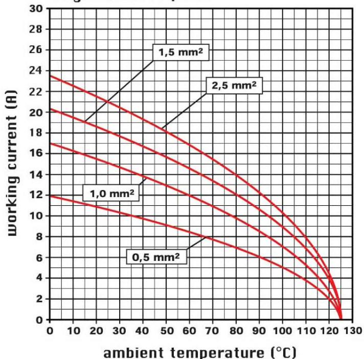
diagram CSH 10 poles
