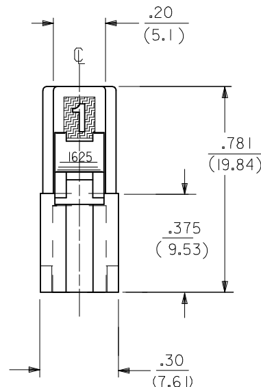
PLUG HOUSING
