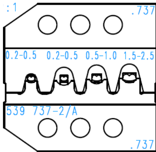
TE 539737-2
