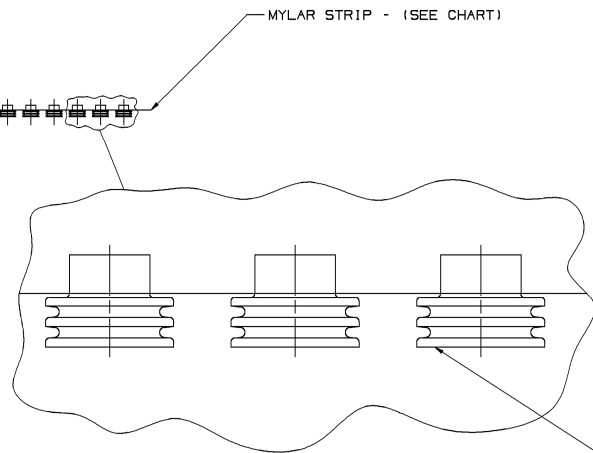
SEAL/MYLAR ASSEMBLY DETAIL
