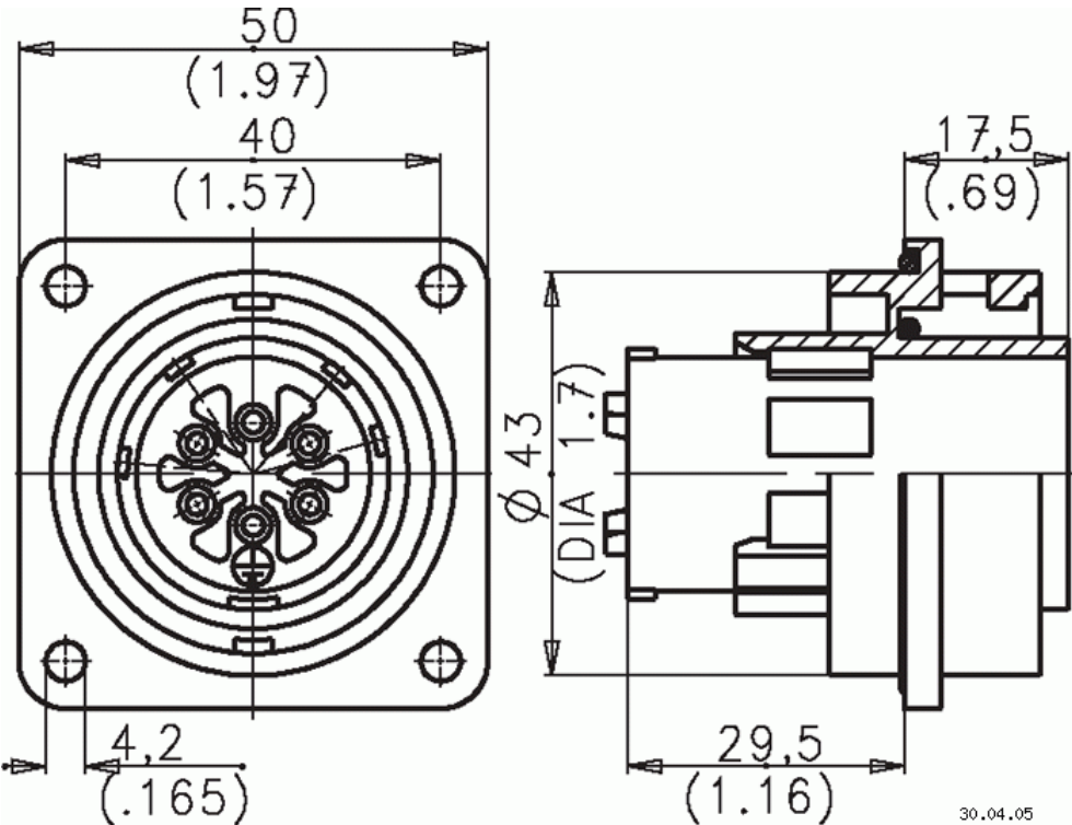
Drawing Dimensions in mm (Inch)
