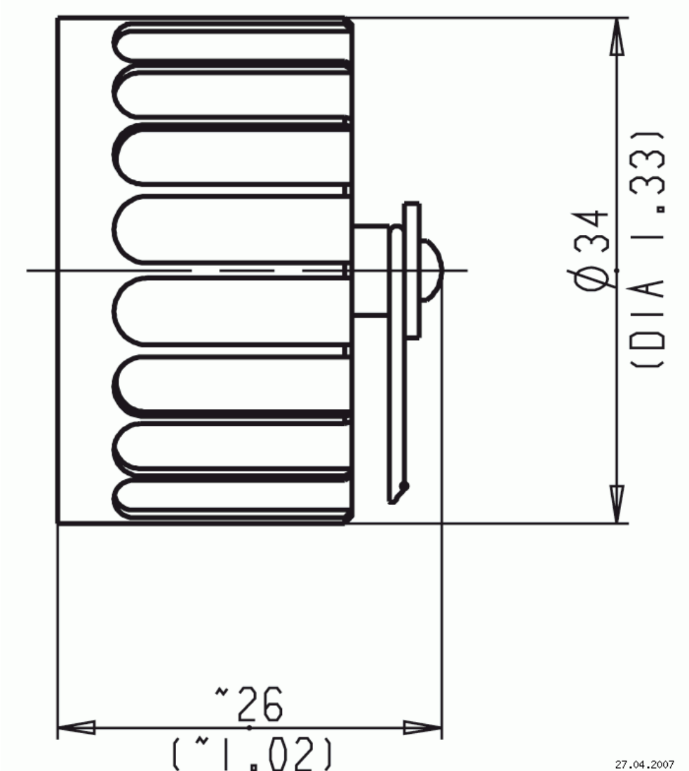
Drawing Dimensions in mm (Inch)
