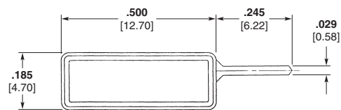
Polarizing Key 1-1437023-2
